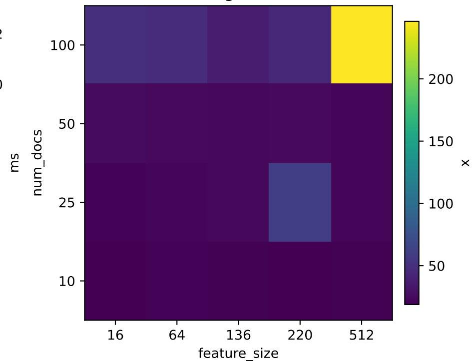
Transformer/LightGBM CPU ratio
